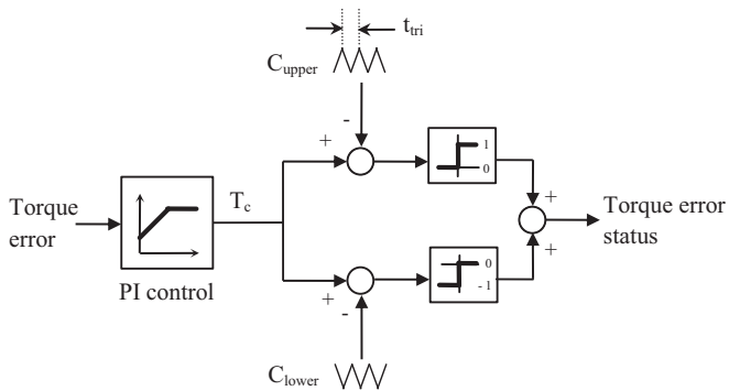
Fig. 6. Constant frequency torque controller (CFTC) [30].
